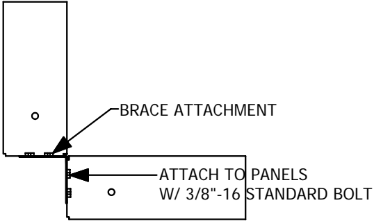
90° CORNER DETAIL OPTIONAL
